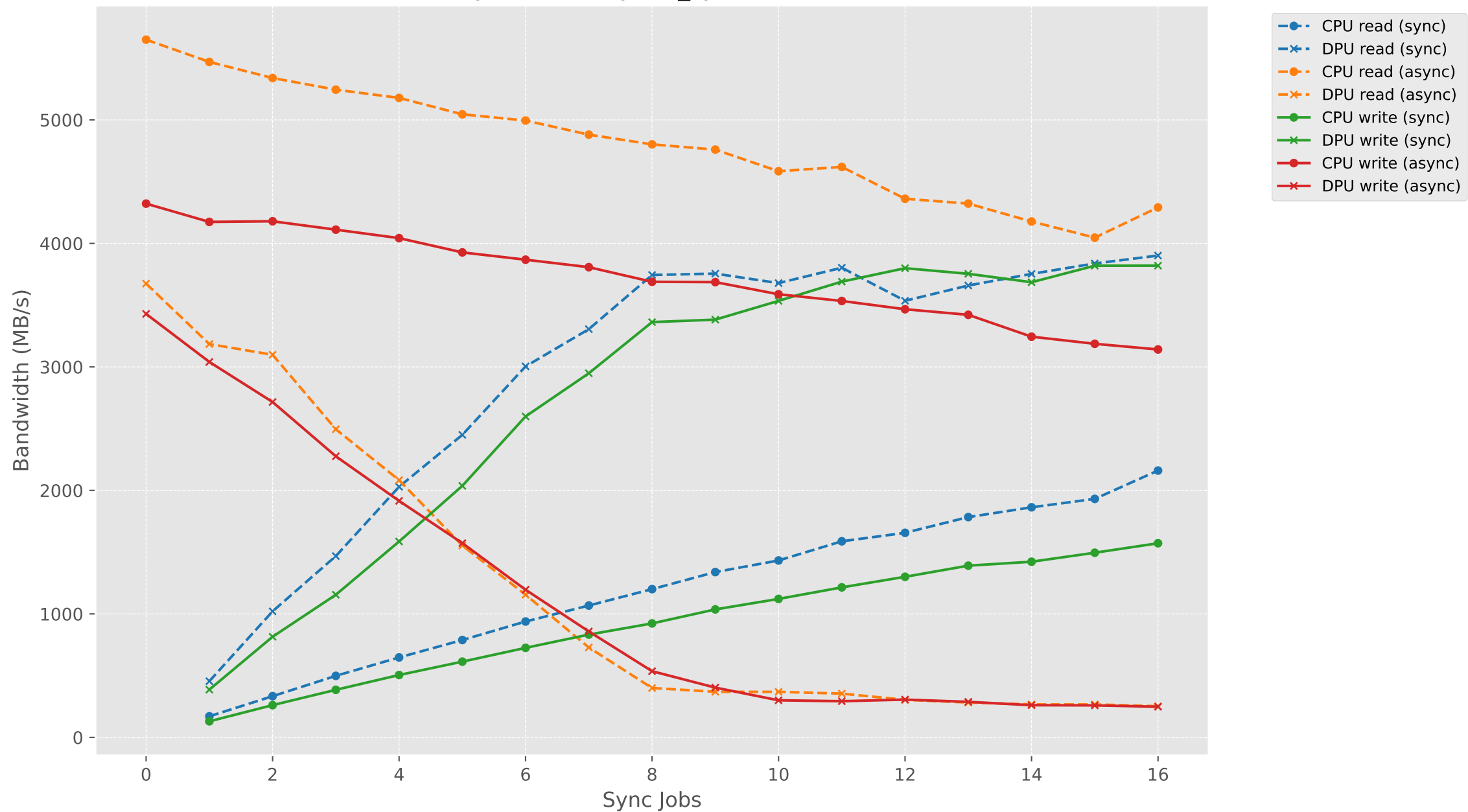
Bandwidth vs Sync Jobs (async1_syncN) - SEQ (CPU vs DPU)
